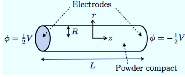
Figure 1: Model set-up considered in this paper. The powder compact is held between two electrodes, at electric potentials \pm\frac{1}{2}V . Radiative and convective heat loss occurs from the free sides of the cylindrical compact, and from the electrodes.
