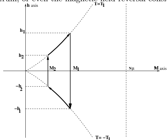
FIG. 1. ‘Carnot’ cycle for a heat pump using negative temperatures. The area enclosed by the loop equals the total energy transferred per cycle. For the nuclear spin system the equation of the temperature- T isotherm is h = (kT/\mu)\text{arctanh}(M/N\mu) . The vertical line at M = N\mu is an asymptote of all the isotherms, both for positive and negative temperatures.
